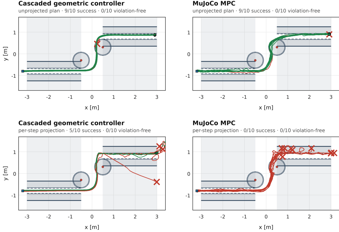
Figure 6.8.: UAV-s-curve from above, drawn like Figure 5.8: FM at K = 1 , ten flights per panel; top, the unprojected plans; bottom, the plans under per-step projection (random selection, tightened constraint set); left, the cascaded geometric controller; right, MuJoCo MPC. Green: success; red: no success; a cross marks a flight that collided or that the divergence guard ended.
